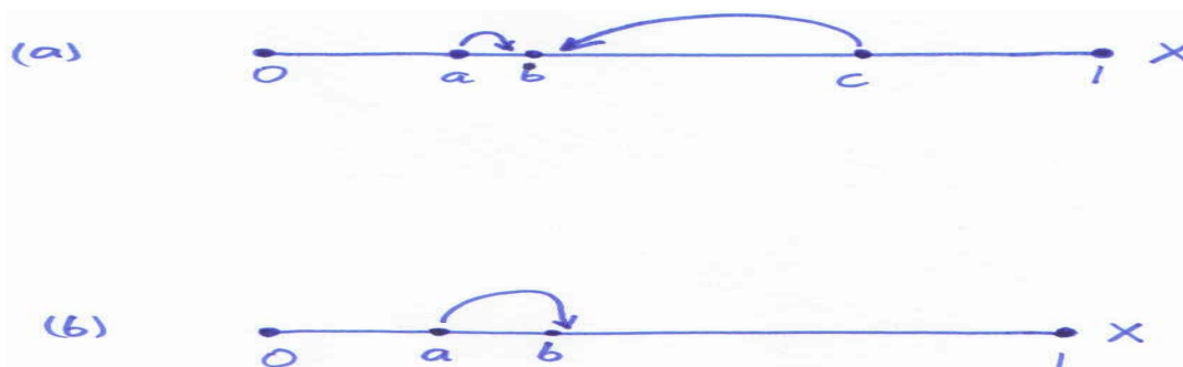
Figure 7: Nonexistence of pure strategies with three players
