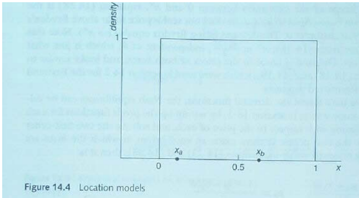
Figure 4: Location Models
