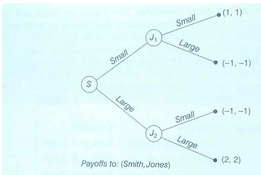
Figure 1: Follow the Leader I
