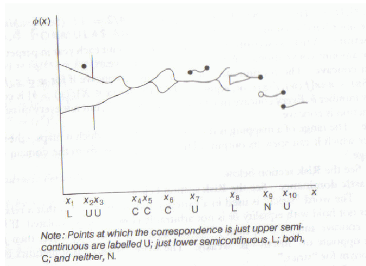
Figure 2 Upper Semicontinuity
