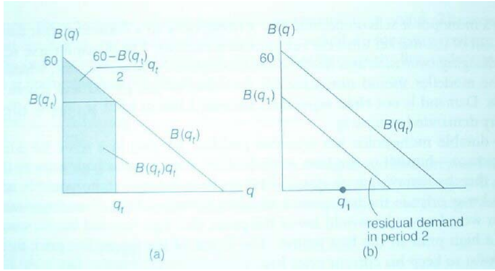
Figure 10: The Buyer's Marginal Benefit per Period in the Game of Durable Monopoly
